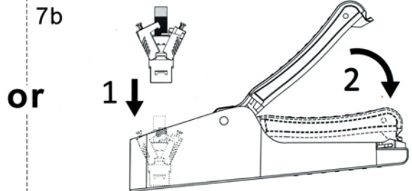
Optional ETC(Easy Tool to Crimp) Tool
